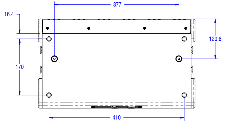
VIEW B-B 94°
